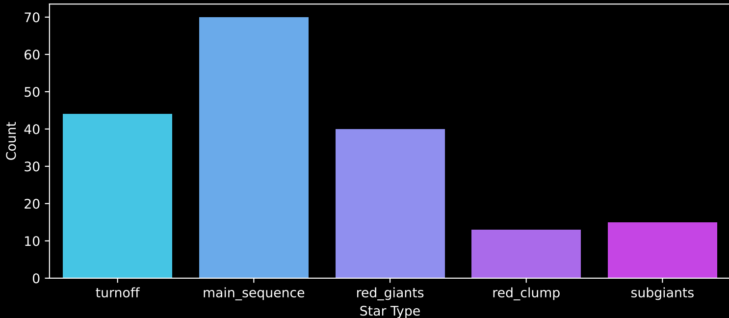
APOGEE DR17 Field: [086+34_MGA] Count plot of Star Type
