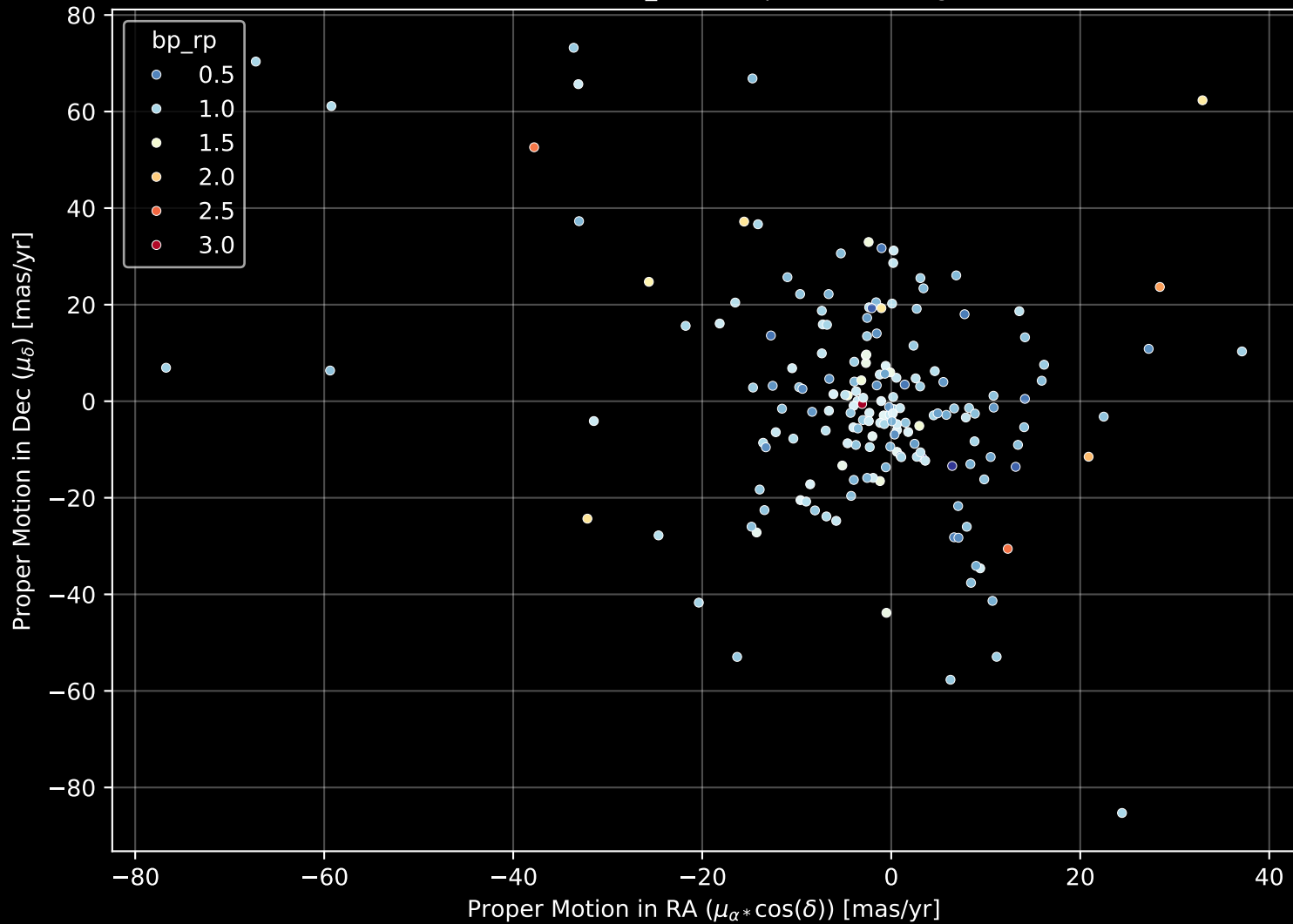
APOGEE DR17 Field: [086+34_MGA] Proper Motion Diagram (n= 182)
