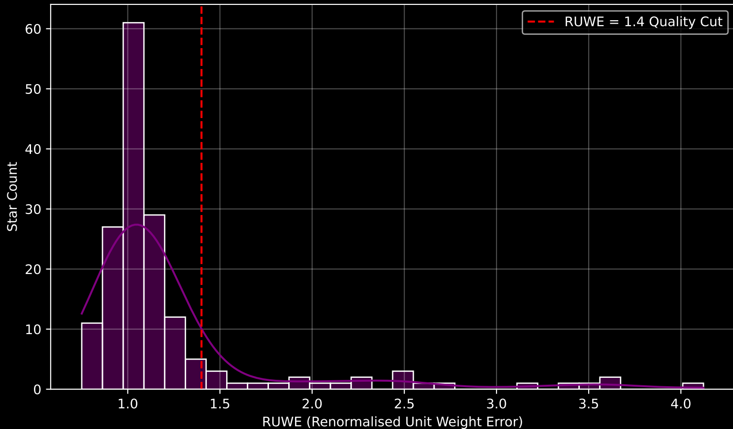
GAPOGEE DR17 Field [086+34_MGA] RUWE Distribution (n= 168)
