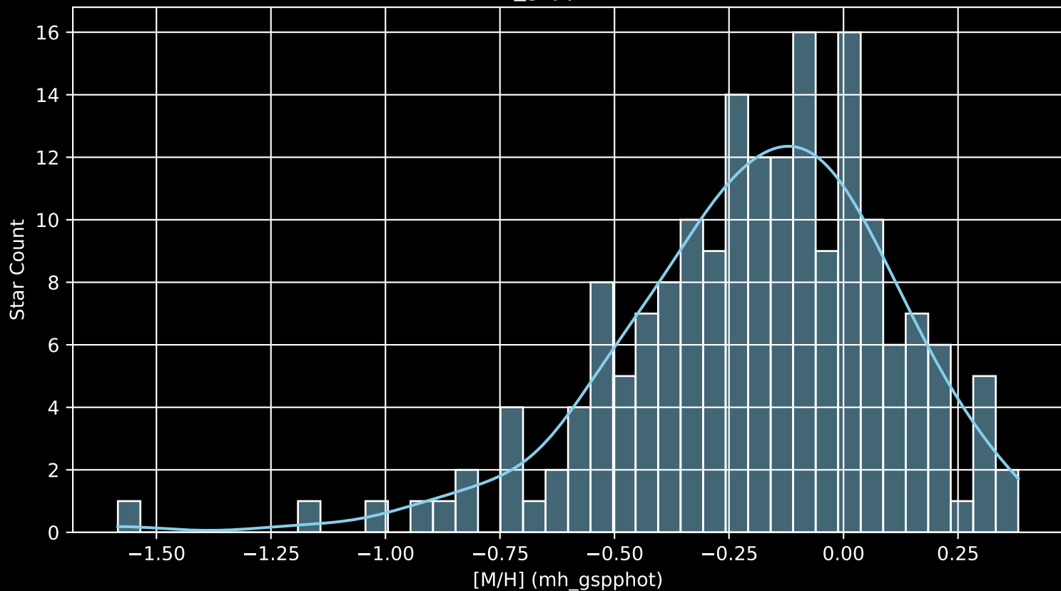
APOGEE DR17 Field: [086+34_MGA [M/H] (mh_gspphot) (n= 181)
