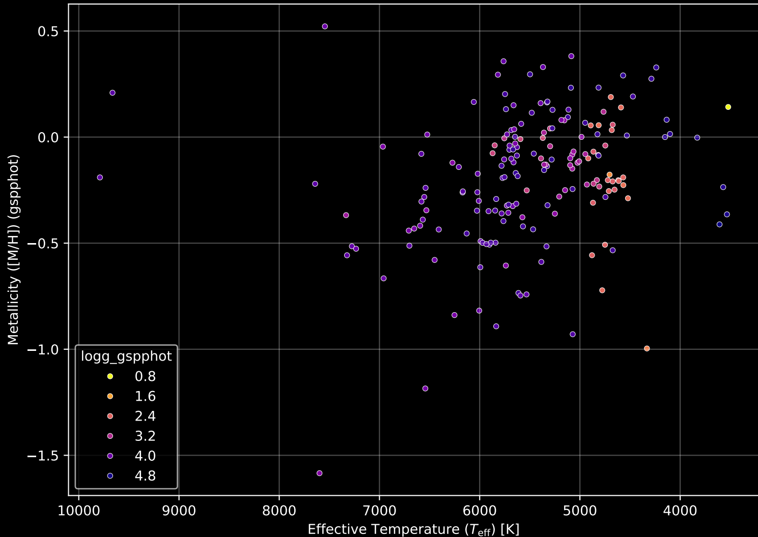
APOGEE DR17 Field: [086+34_MGA] Stellar Population Parameters (n= 182)
