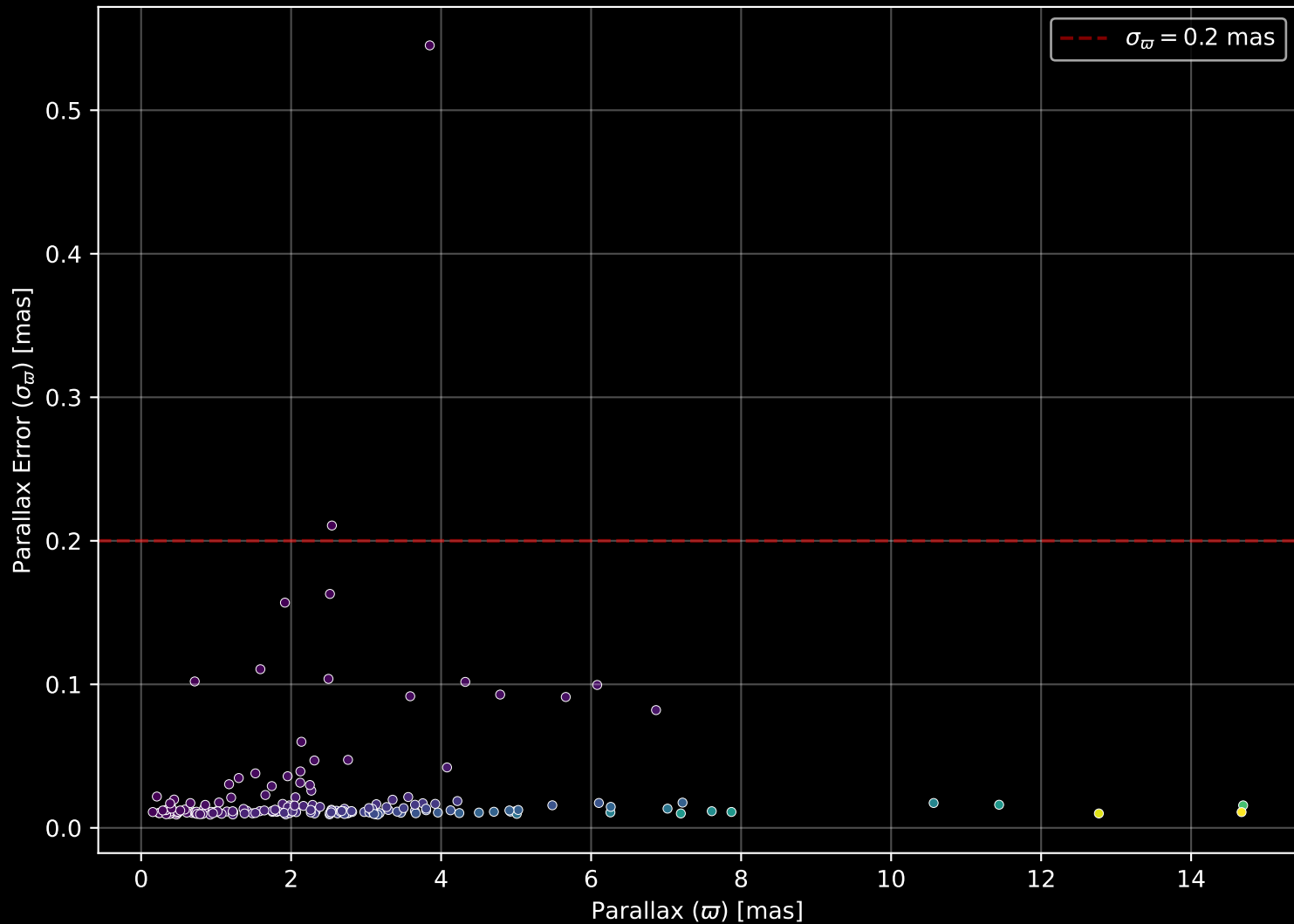
APOGEE DR17 Field: [086+34_MGA] Parallax Quality (n= 182)
